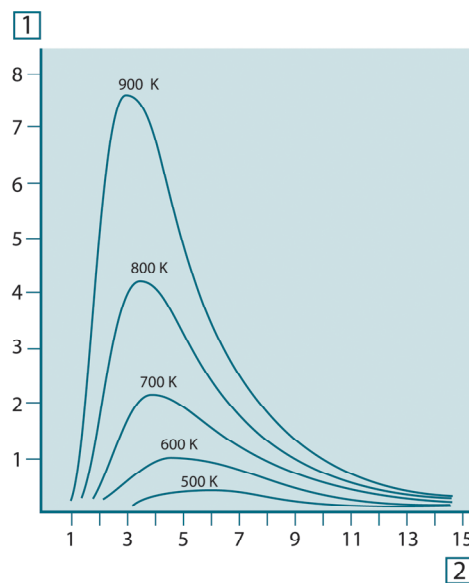
Figure 19.4 Blackbody spectral radiant emittance according to Planck's law, plotted for various absolute temperatures. 1: Spectral radiant emittance (W/cm 2 × 10 3 ( \mu\text{m} )); 2: Wavelength ( \mu\text{m} )
