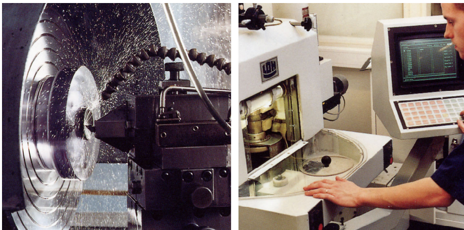
Figure 15.4 LEFT: Diamond turning machine; RIGHT: Lens polishing
